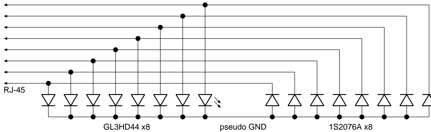
Remote Block
